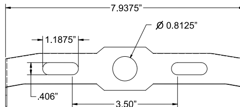
AC-FLA-FM50 (for FFLA50)
