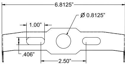
AC-FLA-FM30 (for FFLA30)
